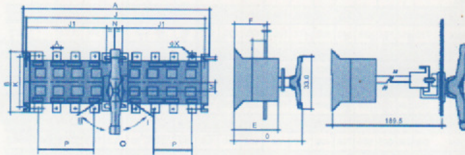
Direct operation on front face GLZ2-125A-1600A
